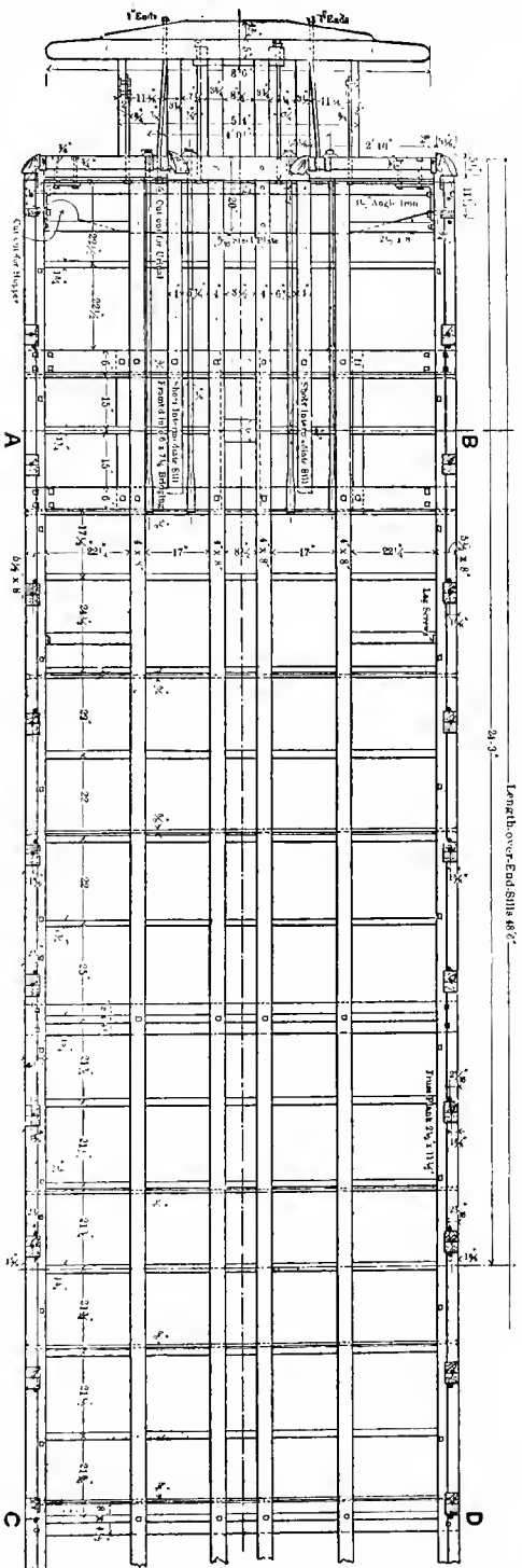
Fig. 456. Part Side Elevation of Framing.
